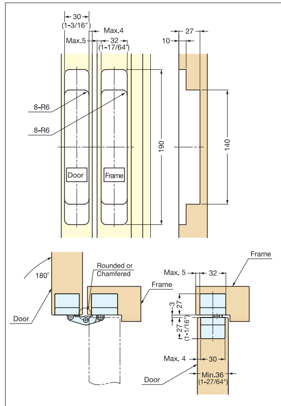
Bore Dimensions
